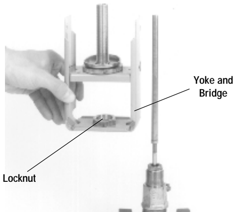
10A. (1/2" TO 2") LIFT OFF BRIDGE/YOKE ASSEMBLY
