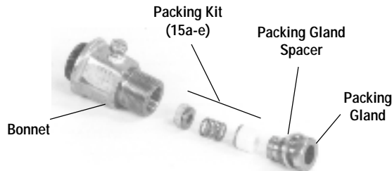
13. PACKING COMPONENTS
