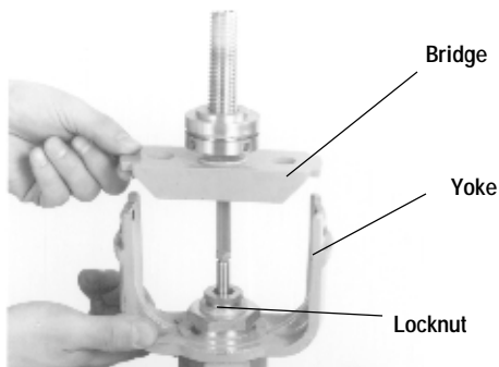
10B. (2-1/2" TO 4") LIFT OFF BRIDGE AND YOKE
