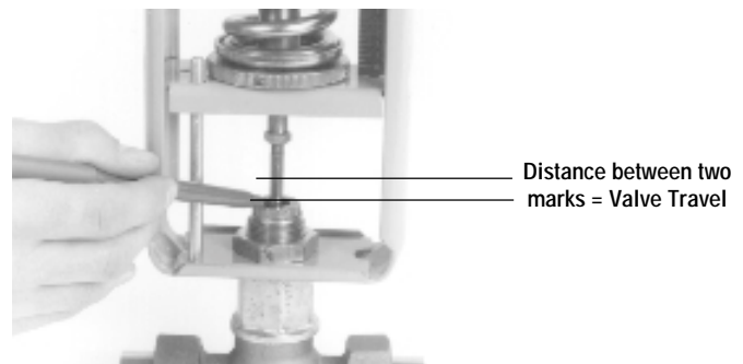
15. VALVE TRAVEL MEASUREMENT
