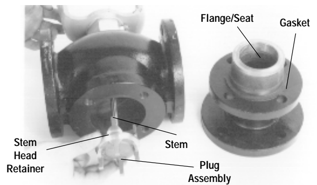
12B. (2-1/2" TO 4") PLUG ASSEMBLY
