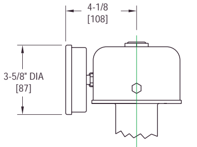
Optional Indicating Head for 1/2" to 2" valves
