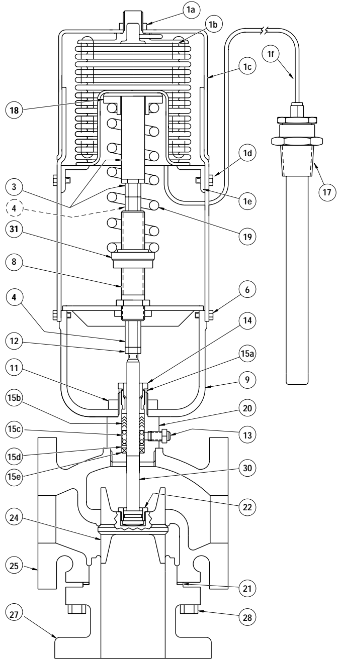
2-1/2" - 4" WM Assemblies
